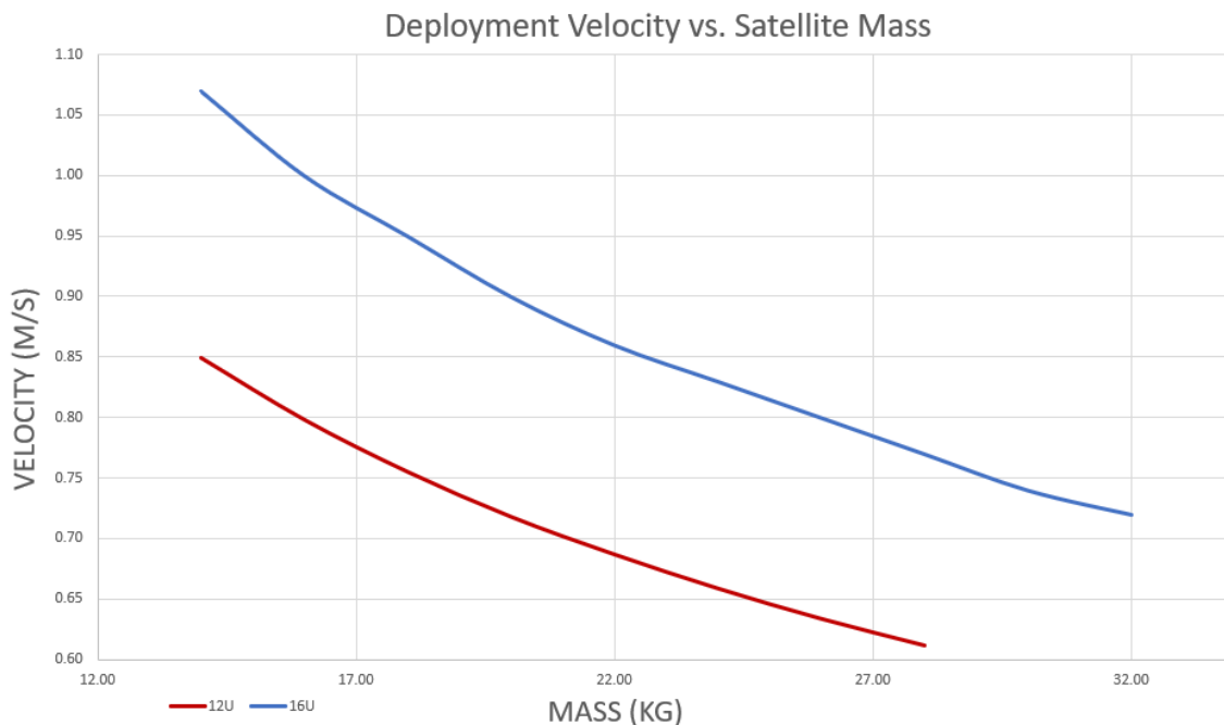
Figure 13: Deployment Velocity
